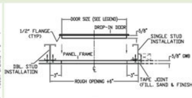
Drop-in Access Panel - Side View (Single/Double stud installation)
